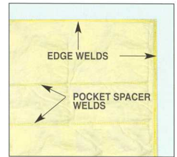
Ultrasonic Welds
